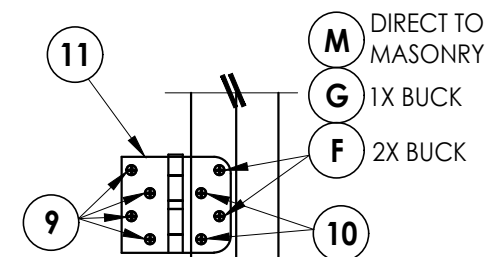
HINGE DETAIL
